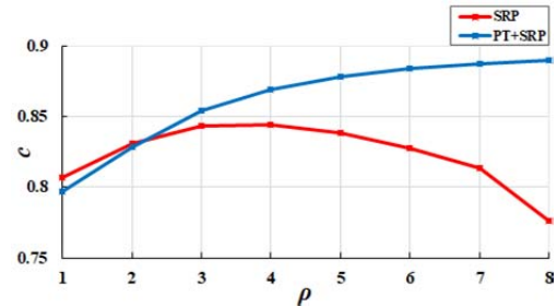
Fig. 12. Comparison between SRP and PT+SRP in terms of the average of the highest correlation costs.
