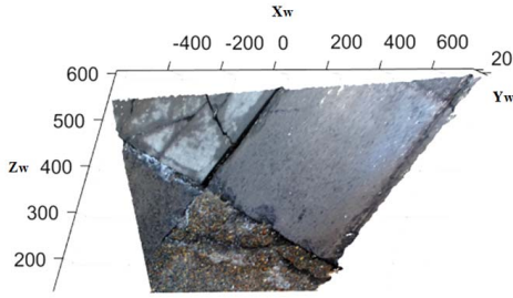
Fig. 8. Road surface 3D reconstruction.
