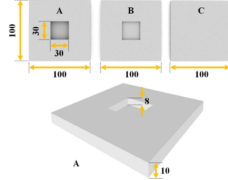
Fig. 10. Designed 3D sample models. The unit is millimeter.
