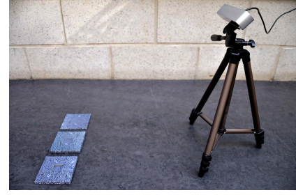
Fig. 9. Experimental set-up.
