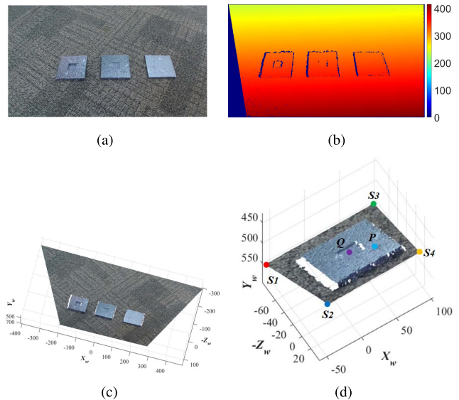
Fig. 15. Sample model 3D reconstruction. (a) left image. (b) subpixel disparity map with post-processing. (c) reconstructed scenery. (d) selected 3D point cloud which includes model B.
