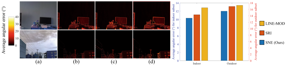
Fig. 3. Qualitative and quantitative results on the DIODE dataset: (a) RGB images; (b)–(d): the angular error maps obtained using our proposed SNE, SRI [2] and LINE-MOD [22], respectively.
