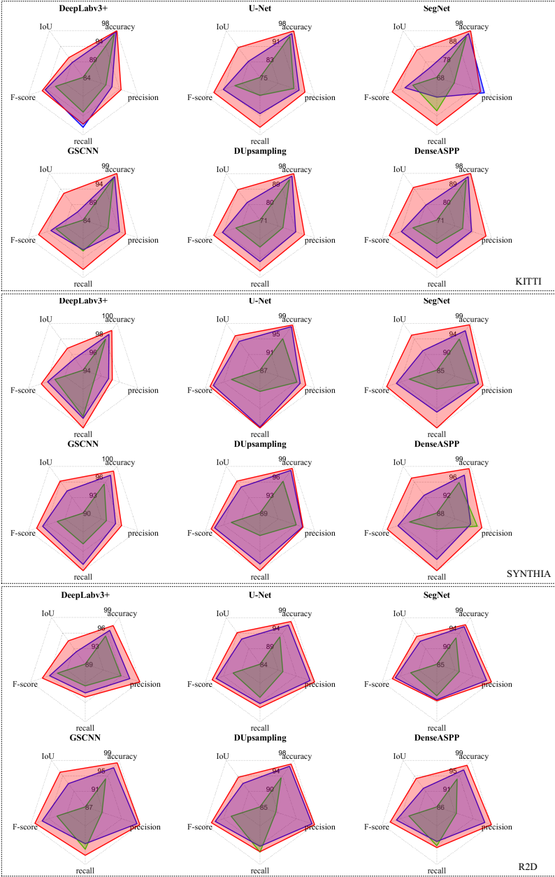
Fig. 5. Performance comparison (%) among DeepLabv3+ [9], U-Net [26], SegNet [3], GSCNN [30], DUpsampling [32] and DenseASPP [37] with and without our SNE embedded, where RGB, Depth, and SNE-Depth (Ours).
